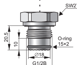
CG1/2 type G1/2" with flush diaphragm Wetted parts materials: 316Lss
