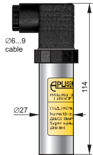
PD type electrical connection, IP-65 Connector DIN 43650
