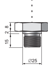
G1/4" Wetted parts materials: 316Lss Min range: 10mbar Max range: 350bar
