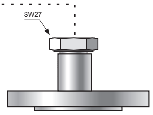
Version with direct or remount mount diaphragm seal. Diaphragm seal data -see chapter III
