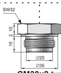
CM30×2 type M30×2 with flush diaphragm
