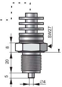
RG type G1/2" with radiator RM type M20×1.5 with radiator Wetted parts materials: 316Lss max. temperature up to 170°C, Min. range 160 mbar Max. range 40 bar
